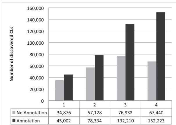
Figure 4: Results of incremental knowledge linking.
