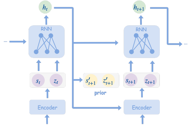
Figure 3: An illustration of the RNN structure in BurstGraph , the hidden variable h_t is updated by last hidden variable h_{t-1} , random variables z_t and s_t . h_0 is set to a zero vector. The prior s'_t and z'_t depend on h_{t-1} . The initial prior s'_0 follows the distribution p^*(s_t) mentioned before, while the initial prior z'_t follows a standard Gaussian distribution.
