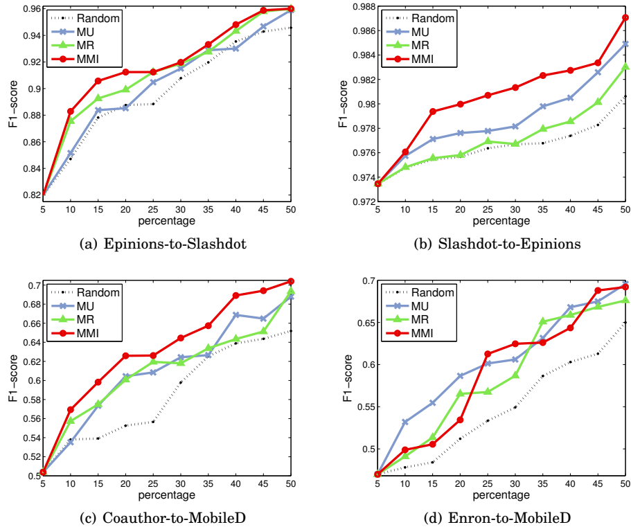
Fig. 2. Performance of active learning. MMI is our proposed method; Random, MU, and MR are three comparison methods.
