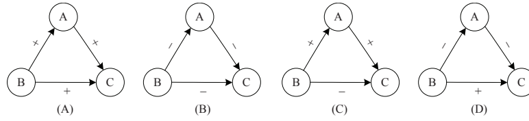
Fig. 7. Illustration of status theory. (A) and (B) satisfy the status theory, while (C) and (D) do not satisfy the status theory. Here positive “+” denotes the target node has a higher status than the source node; and negative “-” denotes the target node has a lower status than the source node. In total there are 16 different cases.
