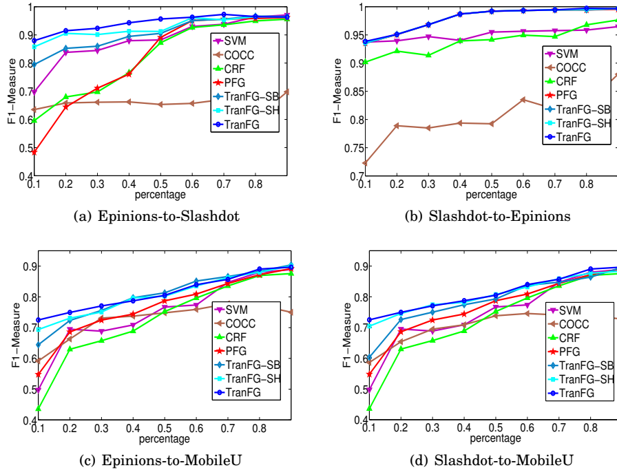
Fig. 14. Performance of predicting friendships with and w/o the balance and structural hole based transfer by varying the percent of labeled data in the target network.
