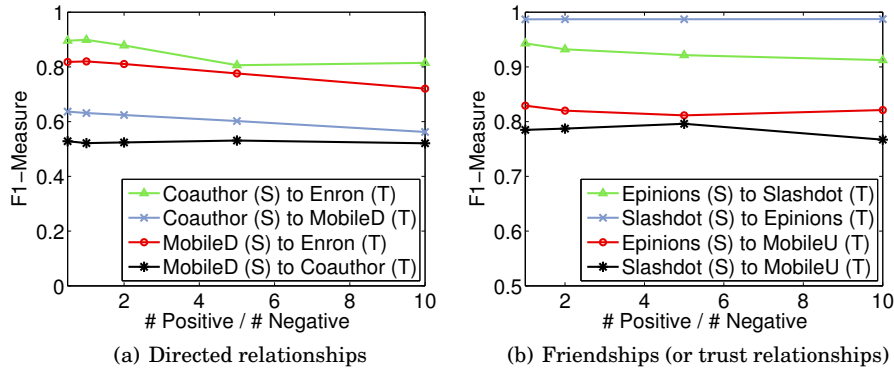
Fig. 12. Bias analysis for transfer link prediction by the proposed TranFG.
