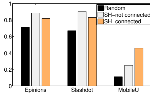
Fig. 6. Structural hole. SH-connected and SH-not connected respectively represents the probability that two connected and two disconnected users (A and B) have the same type of relationship with user C, conditioned on user C spans a structural hole. “Random” indicates the average probability that two users (A and B) have the same type of relationship with user C no matter C spans a structural hole. It is clear that users are more likely (averagely +70% higher than chance) to have the same type of relationship with C if C spans a structural hole.
