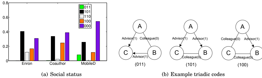
Fig. 8. Distribution of five most frequent formations of triads with social status. Given a triad (A, B, C) , let us use 1 to denote the advisor-advisee relationship and 0 colleague relationship. The number 011 denotes A and B are colleagues, B is C 's advisor and A is C 's advisor.
