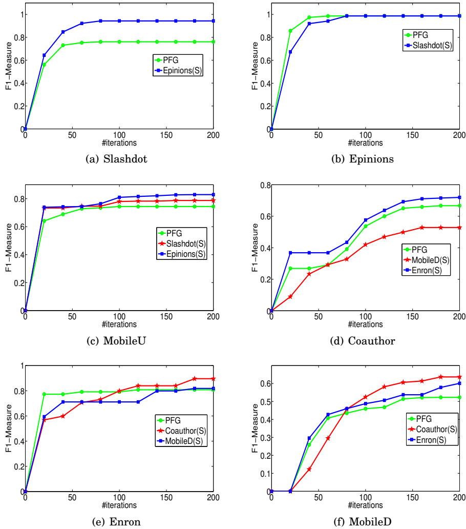
Fig. 16. Convergence analysis of learning algorithm on six different networks.
