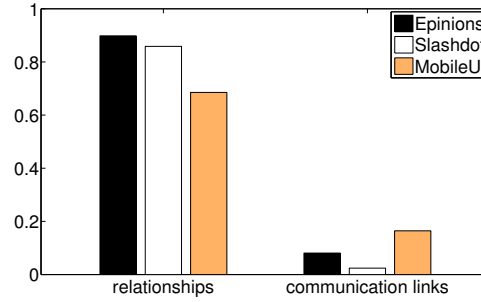
Fig. 5. Social balance. Probabilities of balanced triads in different networks based on communication links and friendships (or trustful relationships). Based on the communication links, different networks have very different balance probabilities (e.g., the balance probability in the mobile network is nearly 7 times higher than that of the slashdot network). Based on friendships, however, the three networks have a relatively similar probabilities.
