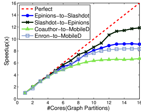
Fig. 3. Speedup vs. #cores.
