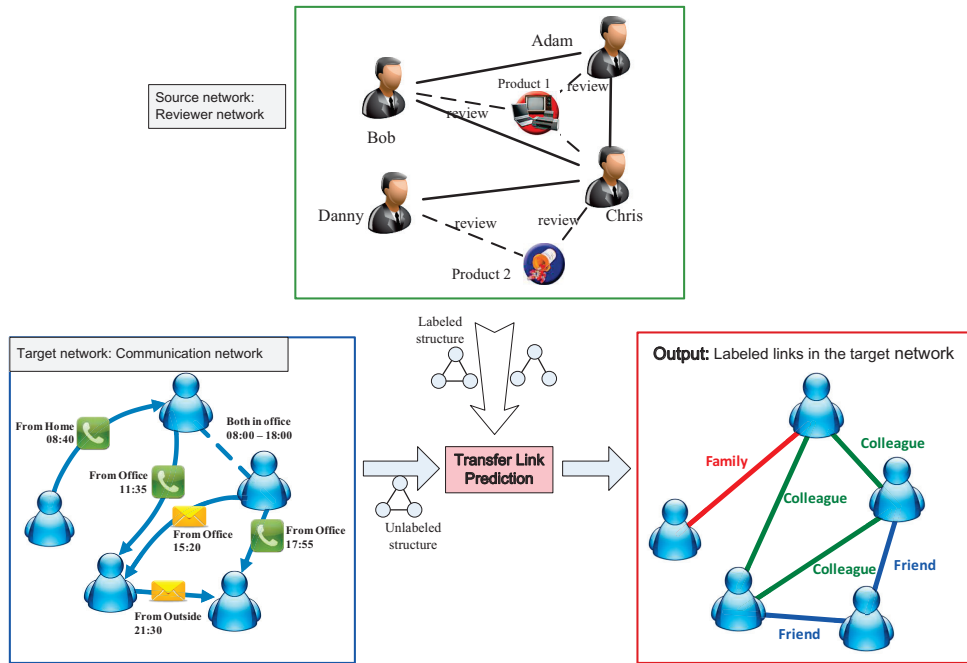
Fig. 1. Example of transfer link prediction across two heterogeneous networks: a reviewer network and a mobile communication network. In our problem setting, given a source network with sufficient labeled relationships and a target network with only a few relationships with labels, our goal is to leverage the labeled relationships/structures in the source network to help predict the type of relationships in the target network.
