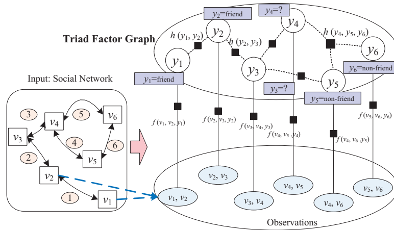
Fig. 11. Graphical representation of the triad factor graph (TriFG) model. Each ellipse indicates a relationship, e.g., (v_1, v_2) represents a relationship between v_1 and v_2 . Notation \mathbf{x}_1 indicates the attribute vector associated with the relationship (v_1, v_2) . For each relationship, we use a corresponding latent variable y denoted as a circle to represent its type. Each black square denotes a factor function which takes the associated variables as input and output a real number.
