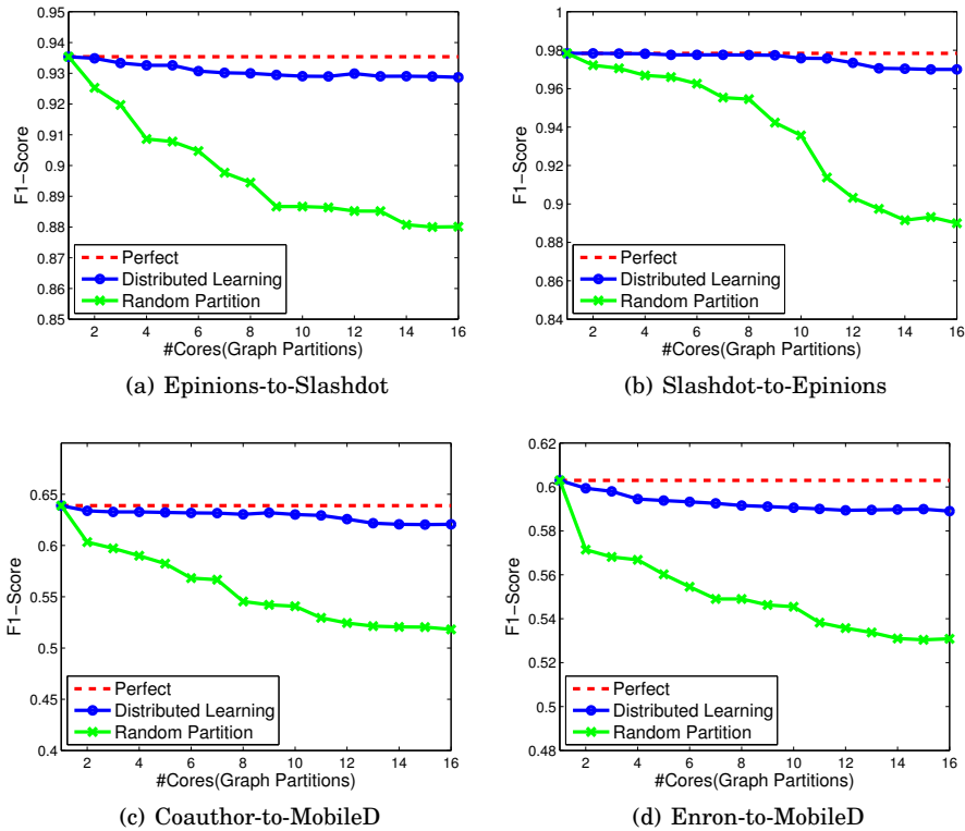
Fig. 17. Prediction accuracy (F1-score) by the distributed learning. The red dash line is the accuracy performance on a single machine.
