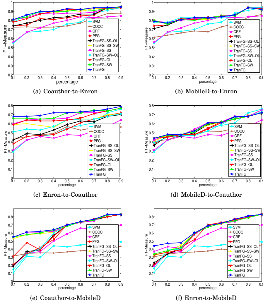
Fig. 15. Performance of predicting directed relationship with and w/o the status, opinion leader, and strong/weak tie based transfer by varying the percent of labeled data in the target network.
