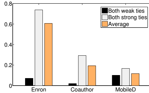
Fig. 10. Strong tie vs. Weak tie. Probabilities of two social ties share the same type, conditioned on whether the two social ties are strong or weak. Average indicates the probability that two random social ties share the same type. It is clear that on all the three data sets, two strong ties result in a higher likelihood to share the same type than chance, while two weak ties are much more uncertain.
