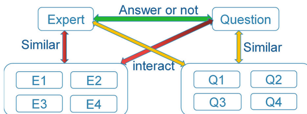
Fig. 1 Implied information
