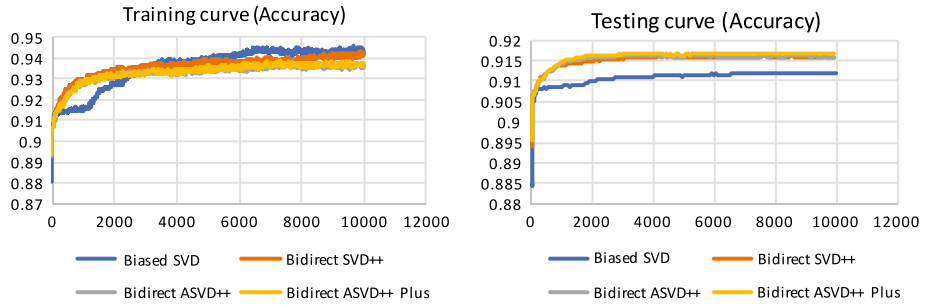
Fig. 4 MF-based models training/testing curve
