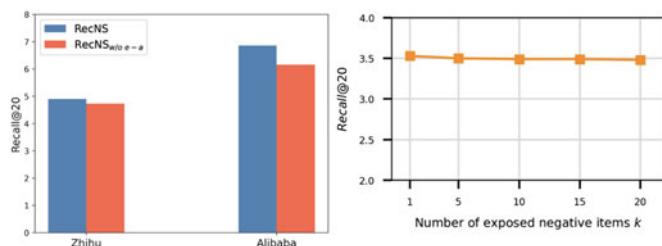
Fig. 9. The impact of the exposure-augmented sampling strategy and the impact of number of sampled exposed negative items.
