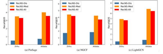
Fig. 7. The impact of the three-region principle.
