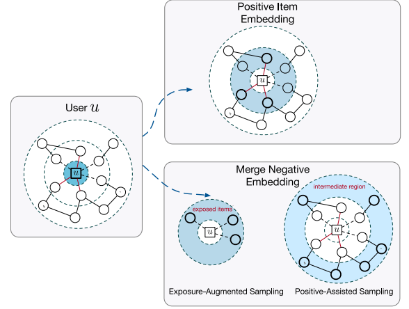
Fig. 1. An illustration of RecNS for merging positive-assisted sampling and exposure-augmented sampling in embedding space.
