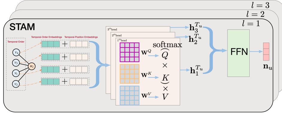
Figure 2: The overall architecture of STAM.
