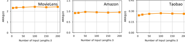
Figure 4: Analyzing the impact of input lengths S on GNN-based recommendation plugged with STAM.
