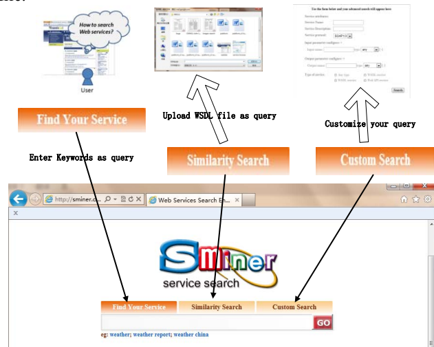
Figure 1. Scenario of Multimodal Query in Web Service Search
