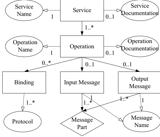
Figure 4. Service Model
