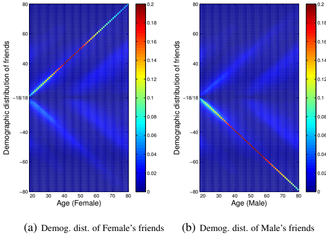
Figure 4: Friends' demographic distribution. X-axis: (a) female age; (b) male age. Y-axis: age of friends (positive: female friends, negative: male friends). The spectrum color represents the friends' demographic distribution.
